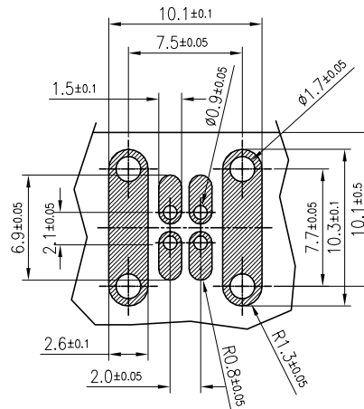
PCBA LAYOUT
