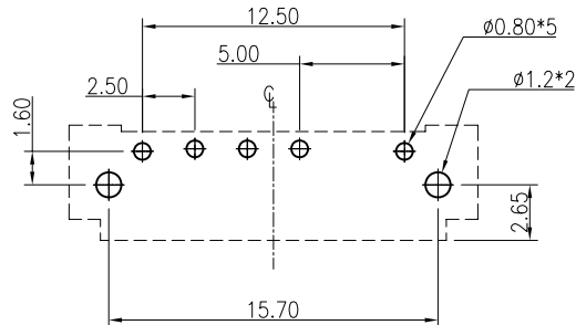
RECOMMENDED PCB LAYOUT GENERAL TOLERANCE \pm 0.05
