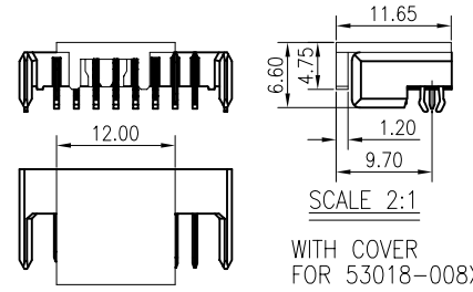
SCALE 2:1 WITH COVER FOR 53018-008XX-001
