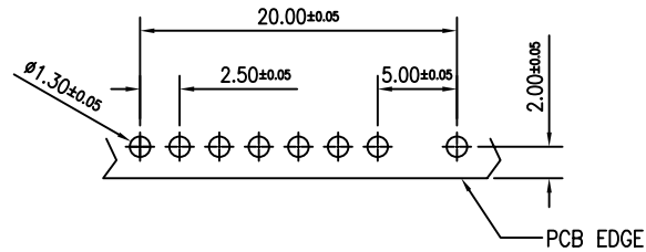
REFERENCE PCB BOARD LAYOUT VIEW FROM CONNECTOR MOUNTING SIDE (PCB THICKNESS=1.2mm)
