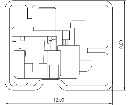
TUBE SECTION
