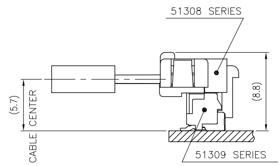
MATED CONDITION
