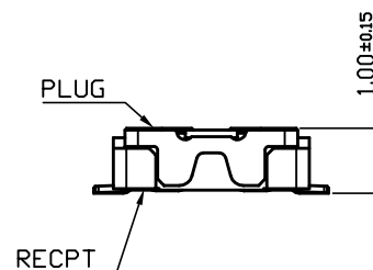
MATING CONDITION
