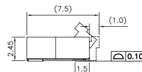
ACTUATOR CLOSED STATE
