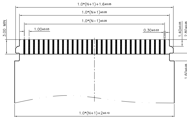
APPLICABLE FPC RECOMMENDED DIMENSION (THICKNESS:0.3±0.03)
