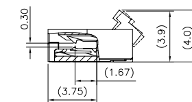
ACTUATOR OPENED STATE
