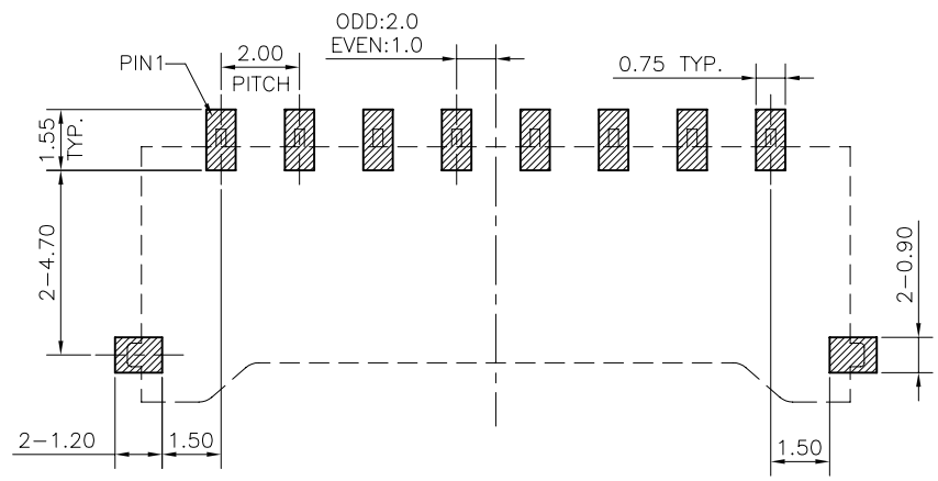
RECOMMEND PCB LAYOUT GENERAL TOLERANCE ±0.05
