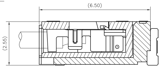
MATING CONDITION (SCALE 2:1)
