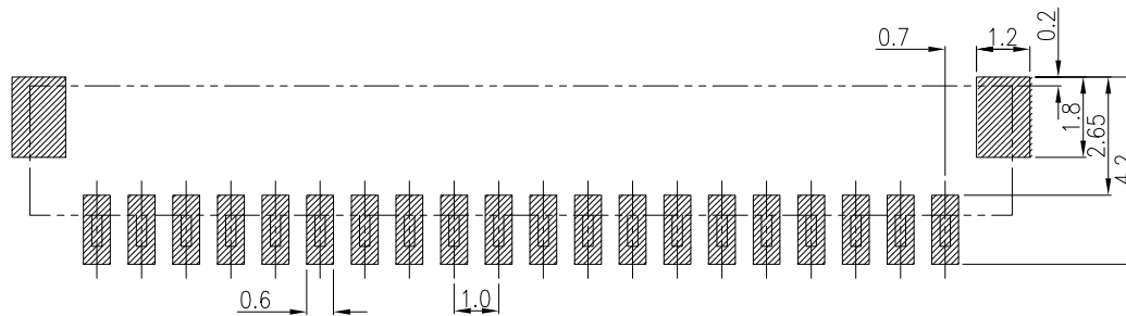
PCB PATTERN LAYOUT
