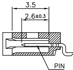
SEC. Y-Y
