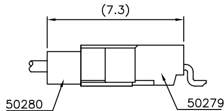
MATED CONDITION
