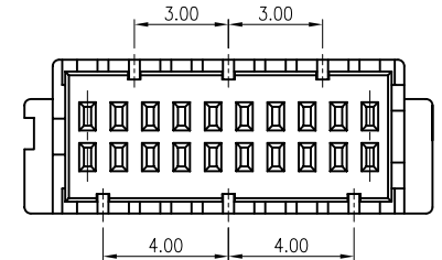
20 PIN
