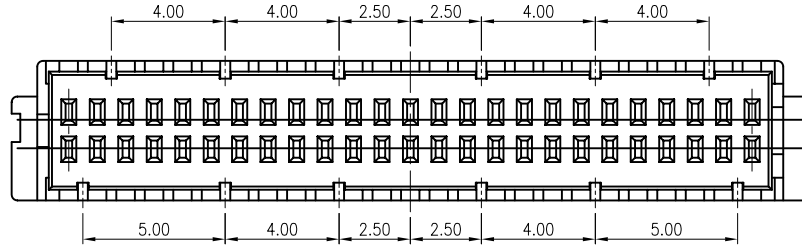
50 PIN
