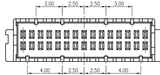
30 PIN
