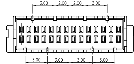
28 PIN
