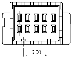
10 PIN
