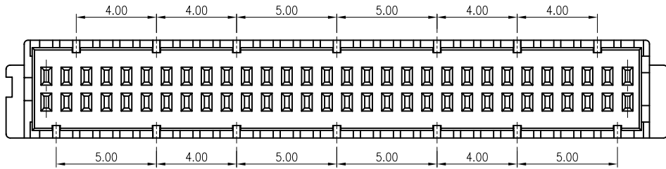
60 PIN
