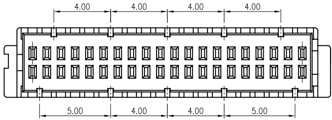
40 PIN
