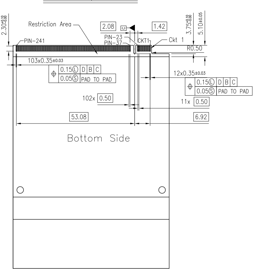
Bottom Side Option one Pad
